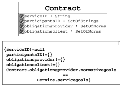
Fig. 7. Class Contract
