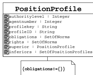
Fig. 8. Class PositionProfile
